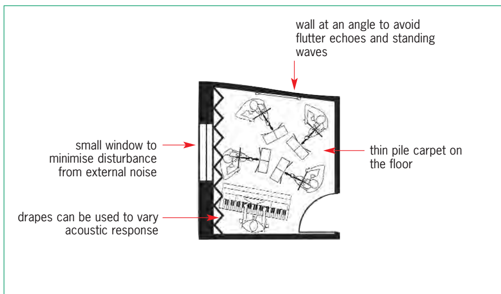
Figure 5.10: Acoustic treatment to 8 m² group room
